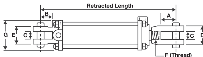
Dimensional Data for Wolverine Cylinders
